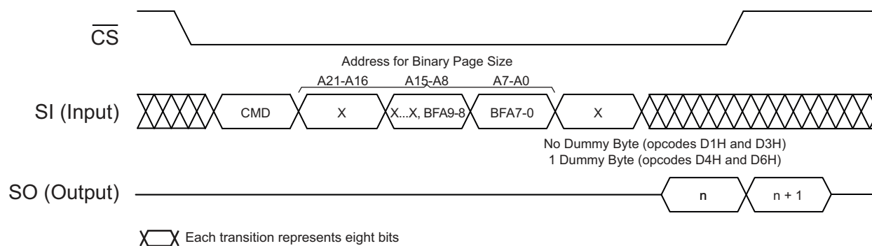
Figure 23-4. Buffer Read
