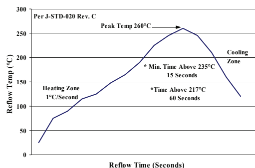
Figure 51. Recommended linear reflow profile using Sn/Ag/Cu solder.
