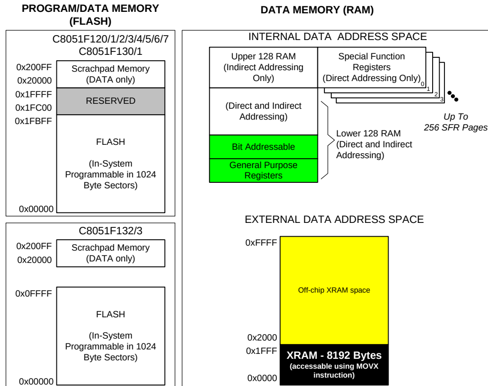
Figure 11.2. Memory Map
