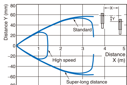
Through-beam E32-T16J
