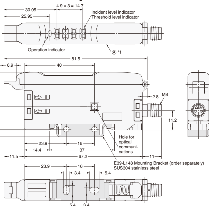
With Mounting Bracket Attached
