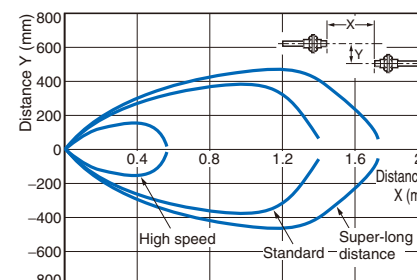
Through-beam E32-T22S
