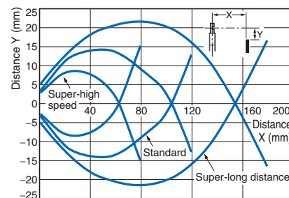
Reflective E32-D61
