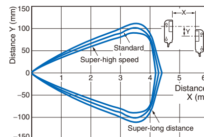
Through-beam E32-T16JR
