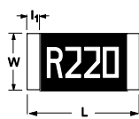
Fig. 6 Chip resistor dimensions
