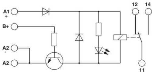
Circuit diagram
