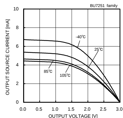
Fig. 9 Output Source Current – Supply Voltage ( V_{DD}=3[V] )
