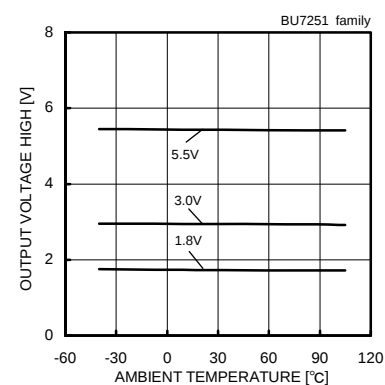
Fig. 6 Output Voltage High – Ambient Temperature ( R_L=10[k\Omega] )
