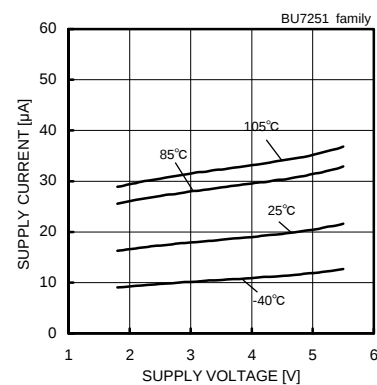
Fig. 3 Supply Current – Supply Voltage
