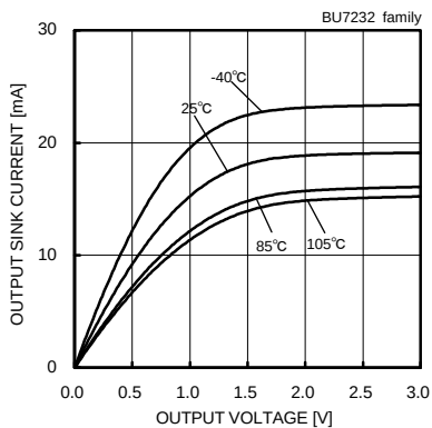
Fig. 77 Output Sink Current – Output Voltage ( V_{DD}=3[V] )
