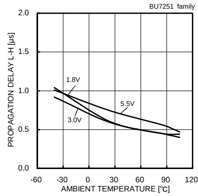
Propagation Delay L-H – Ambient Temperature
