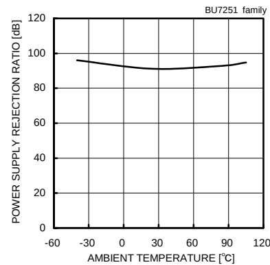
Power Supply Rejection – Ambient Temperature
