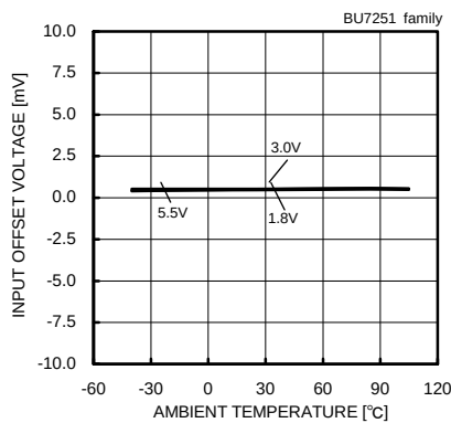
Input Offset Voltage – Ambient Temperature ( V_{cm}=V_{DD} , V_{out}=0.1[V] )
