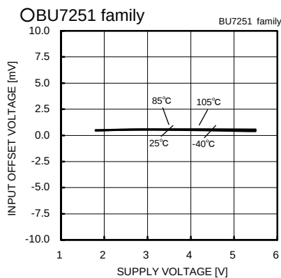
Input Offset Voltage – Supply Voltage ( V_{cm}=V_{DD} , V_{out}=0.1[V] )
