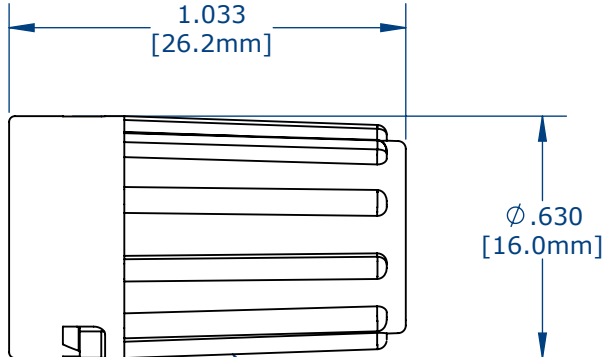
BACKSHELL, LONG
