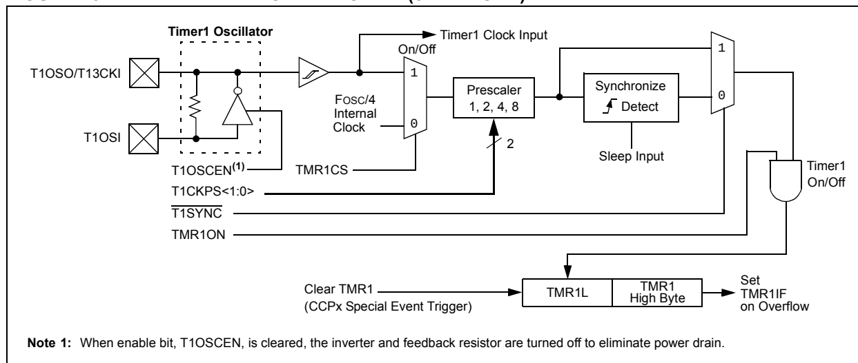
FIGURE 13-1: TIMER1 BLOCK DIAGRAM (8-BIT MODE)
