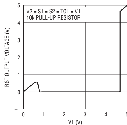
\overline{\text{RST}} Output Voltage vs V1
