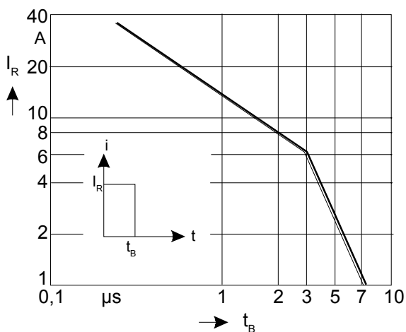
Fig. 10 Maximum peak value of the reverse current admissible for a given pulse-width t_B , which is required for the suitable fast recovery series-diode.
