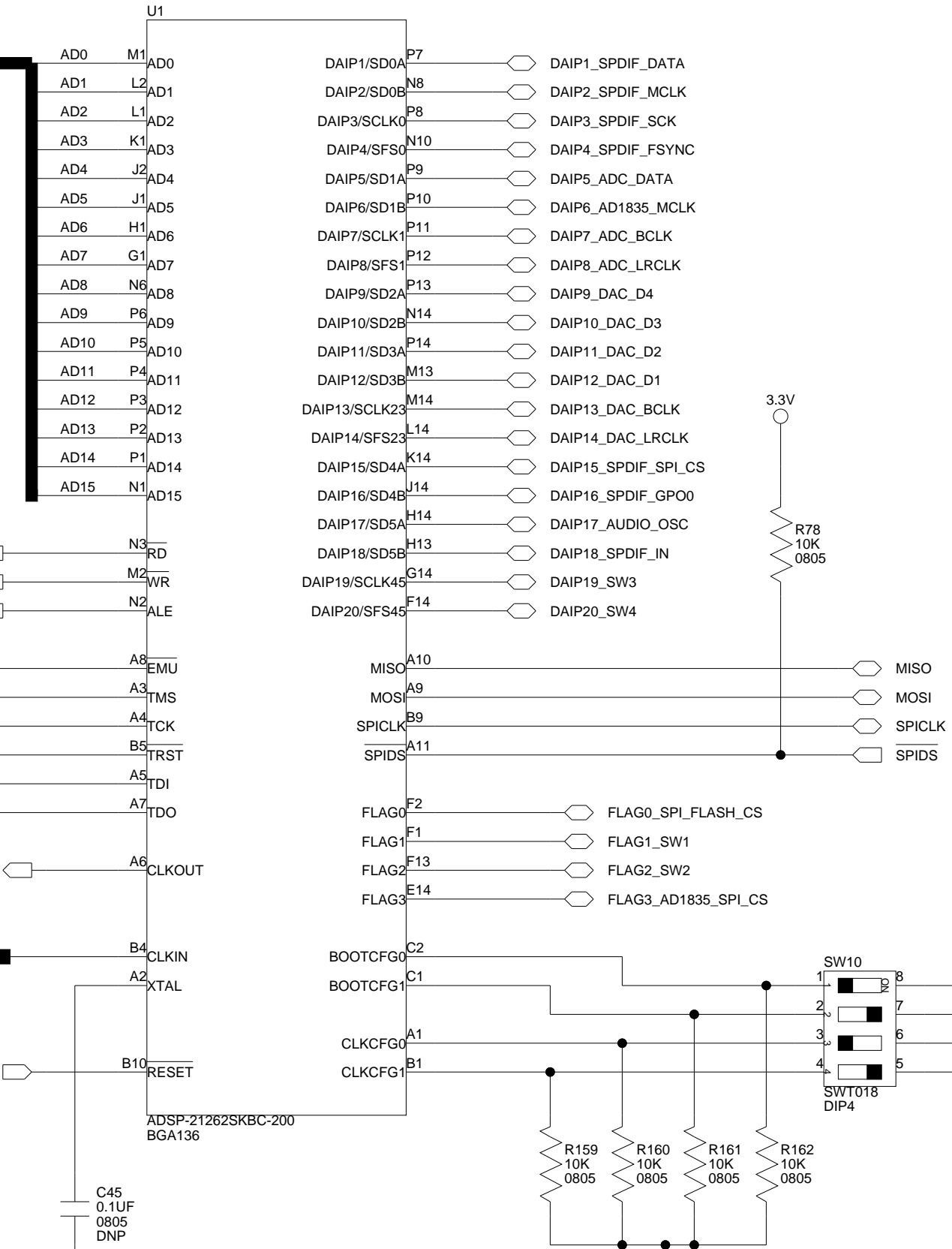
SW10: BOOT/CLOCK RATIO SELECT (Default: 1=OFF, 2=ON, 3=OFF, 4=ON)
