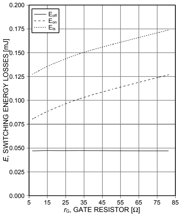
Figure 13. Typical switching energy losses as a function of gate resistor (inductive load, T_{vj}=150^\circ\text{C} , V_{CE}=400\text{V} , V_{GE}=15/0\text{V} , I_C=4\text{A} , Dynamic test circuit in Figure E)
