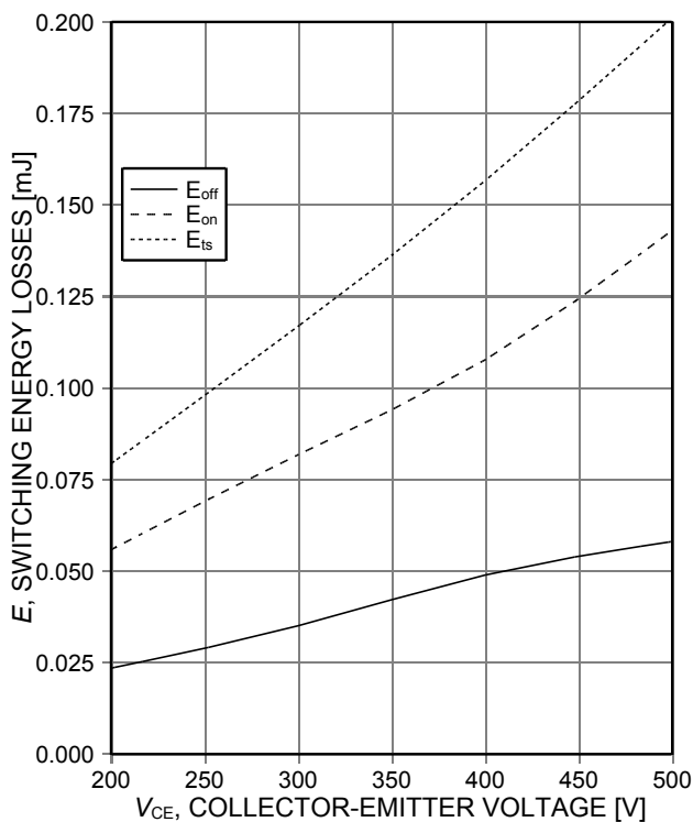
Figure 15. Typical switching energy losses as a function of collector emitter voltage (inductive load, T_{vj}=150^\circ\text{C} , V_{GE}=15/0\text{V} , I_C=4\text{A} , r_G=48\Omega , Dynamic test circuit in Figure E)
