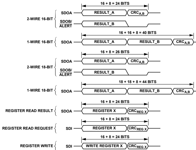
Figure 43. CRC Operation
