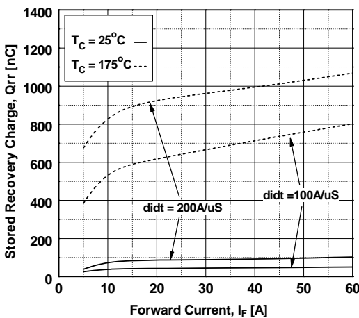
Figure 23. Stored Charge
