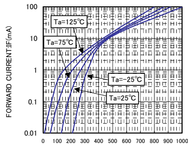
FORWARD VOLTAGE:VF(mV) VF-IF CHARACTERISTICS VF分布
