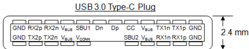
Figure 4-5. USB Type-C Plug Interface (Front View)
