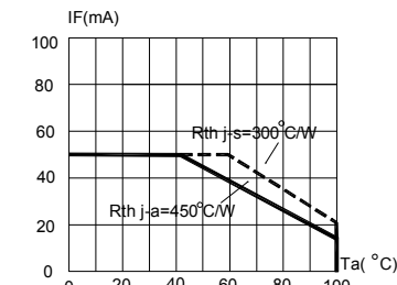
FIG.5 RED&AMBER MAXIMUM FORWARD DC CURRENT VS AMBIENT TEMPERATURE (Tjmax=110°C)
