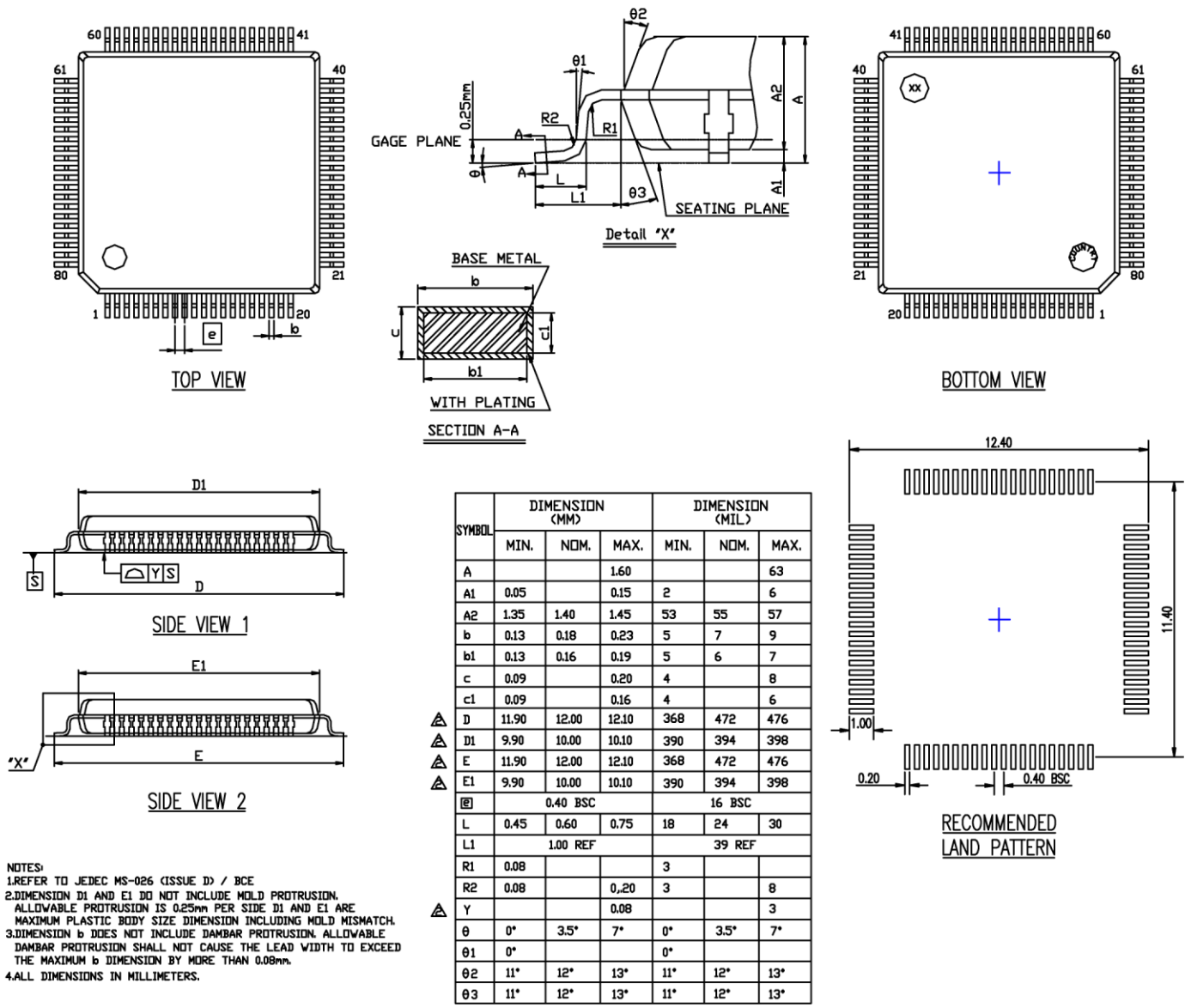
Figure 30. 80-Pin LQFP
