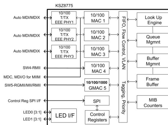
Figure 1. KSZ8775CLX Functional Block Diagram
