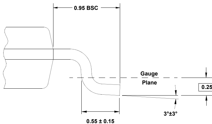
DETAIL "X"
