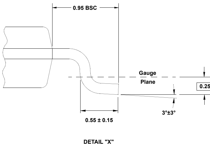
DETAIL "X"
