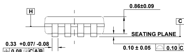
SIDE VIEW 1
