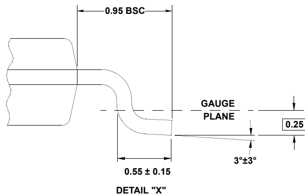
DETAIL "X"
