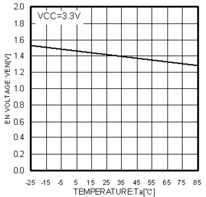
Fig.77 T_a - V_{en}
