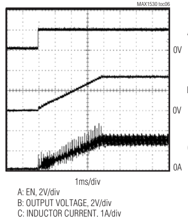
STEP-DOWN REGULATOR SOFT-START
