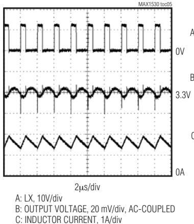
STEP-DOWN REGULATOR SWITCHING WAVEFORM
