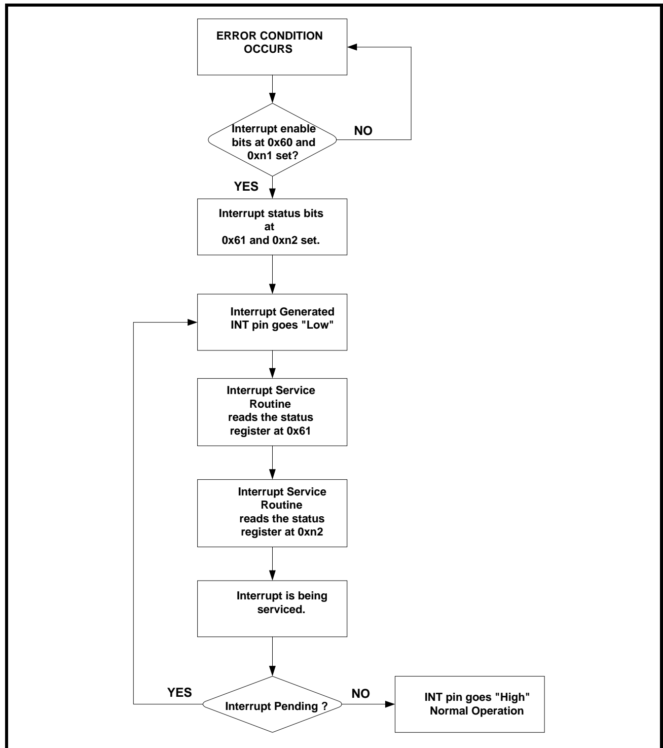
FIGURE 38. INTERRUPT PROCESS
