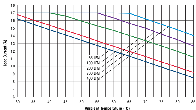
Maximum Power Temperature Derating at Sea Level Vin = 48 (air flow from Pin 1 to Pin 3 on PCB, no baseplate)
