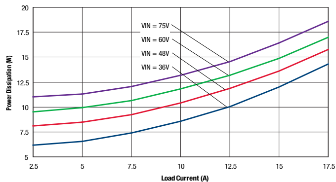
Power Dissipation vs. Load Current @ Ta = +25°C
