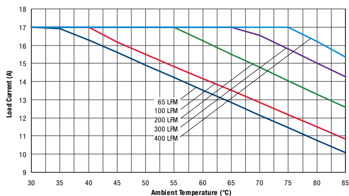
Maximum Power Temperature Derating at Sea Level Vin = 48 (air flow from Pin 1 to Pin 3 on PCB, with baseplate)
