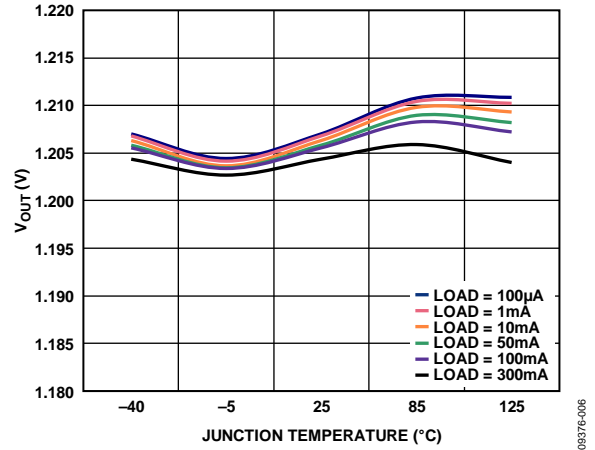
Figure 26. Output Voltage vs. Junction Temperature, V_{OUTx} = 1.2 V , ADP223/ADP225
