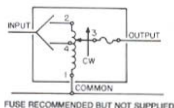
FUSE RECOMMENDED BUT NOT SUPPLIED
