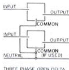
THREE PHASE OPEN DELTA
