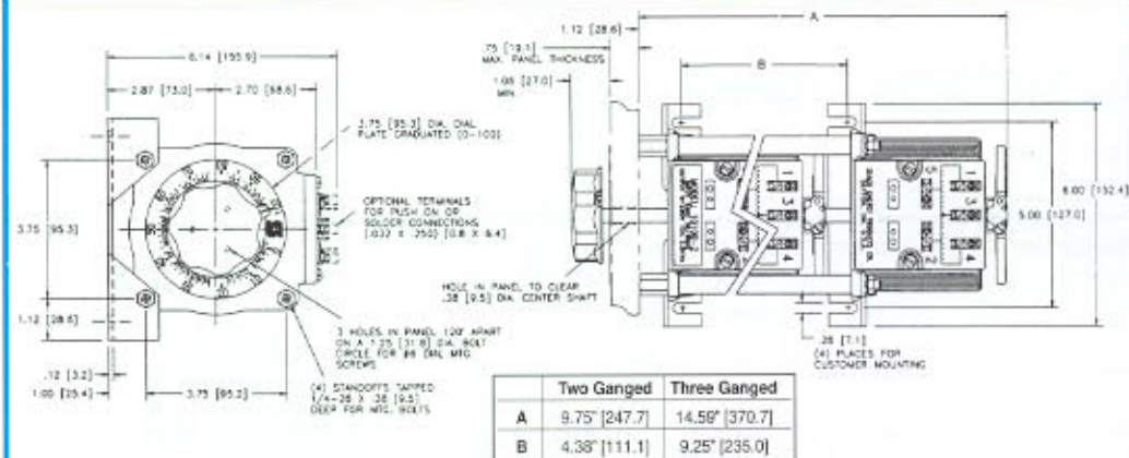
Two and Three Ganged, Uncased
