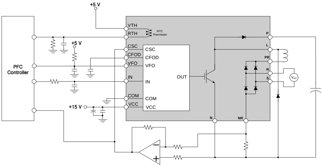
Fig. 9. Application Example
