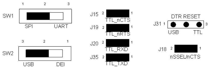
Figure 4. Jumper settings for SPI-mode USB RS-232 serial communication
