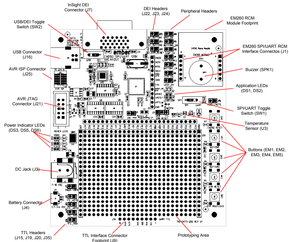
Figure 2. Top side components
