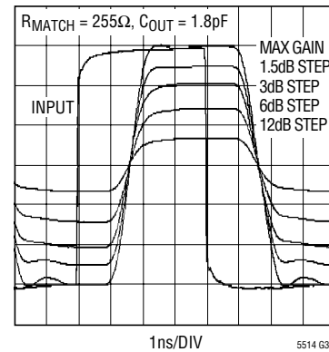
Pulse Response vs Attenuation, LT5514 Levels are: V_{IN} = 66mV_{P-P} , V_{OUT} = 4V_{P-P} at Max Gain
