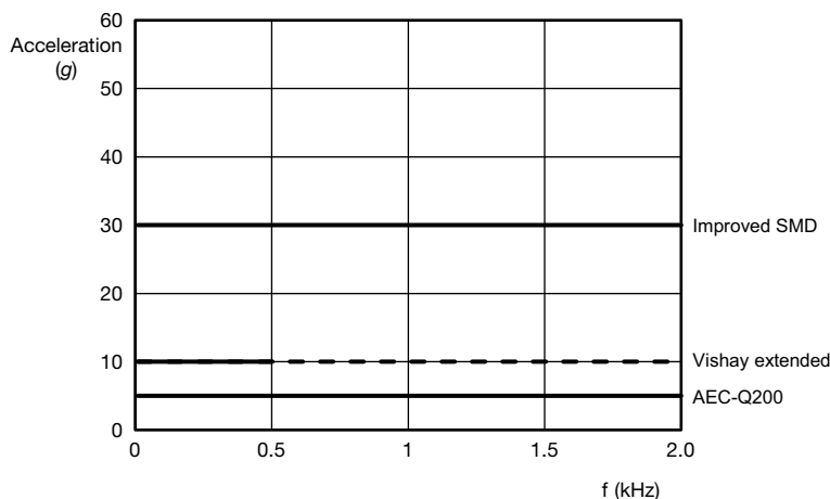
Fig. 4 - Vibration profile
