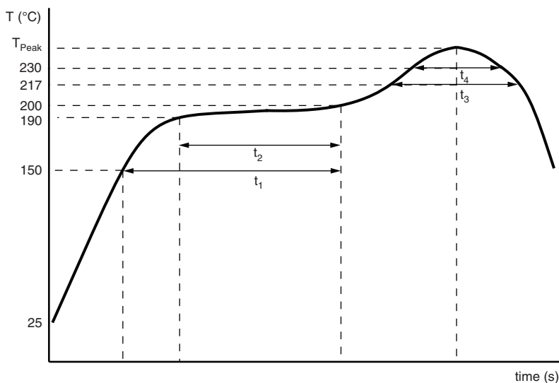
Fig. 3 - Maximum temperature load during reflow soldering
