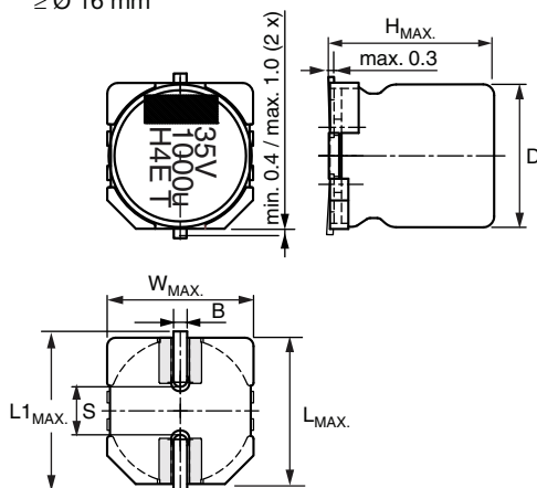
Fig. 1 - Dimensional outline
