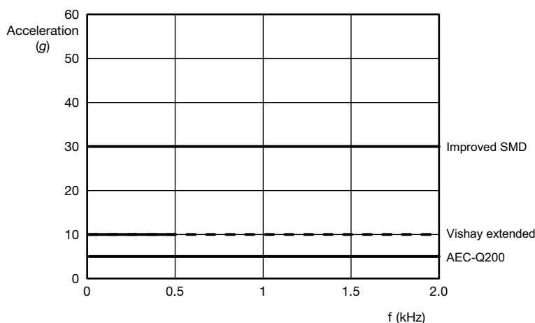
Fig. 4 - Vibration profile
