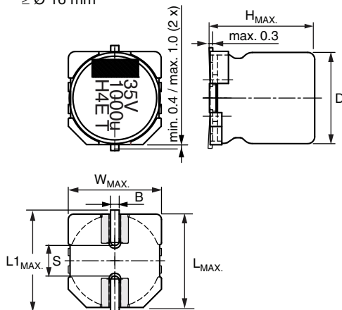
Fig. 1 - Dimensional outline
