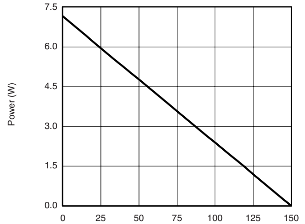
Power Derating, Junction-to-Foot
