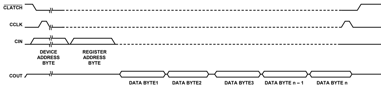
Figure 45. SPI Read from ADAU1977 (Multiple Bytes)
