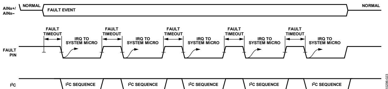
Figure 23. Diagnostics Sequence
