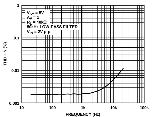
Figure 60. THD + N vs. Frequency
