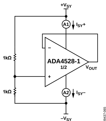
Figure 65. Voltage Follower
