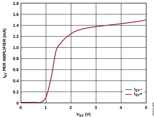
Figure 69. Supply Current vs. Supply Voltage (Comparator A and Comparator B)
