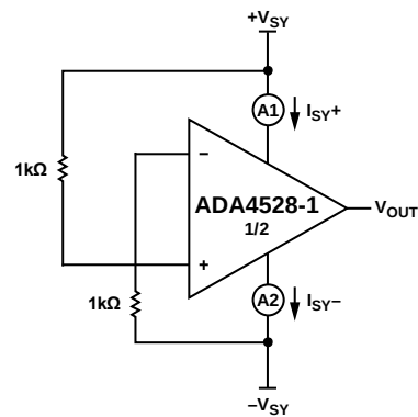
Figure 68. Comparator B
