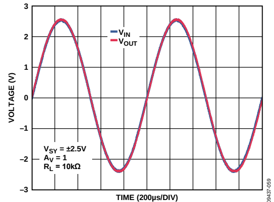
Figure 61. Rail-to-Rail Input and Output
