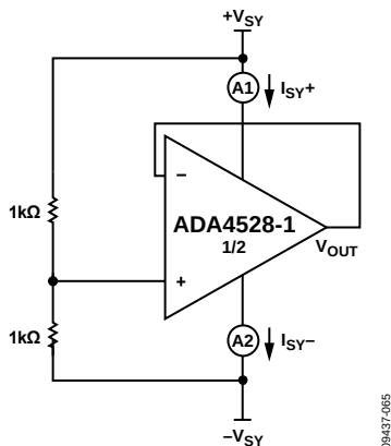
Figure 65. Voltage Follower
