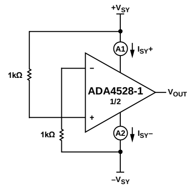
Figure 68. Comparator B
