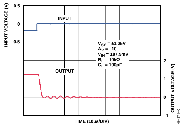
Figure 43. Positive Overload Recovery
