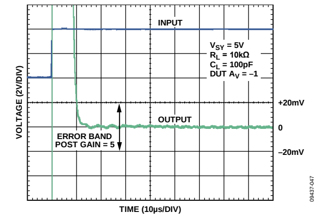
Figure 48. Positive Settling Time to 0.1%
