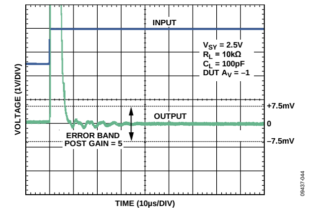
Figure 45. Positive Settling Time to 0.1%
