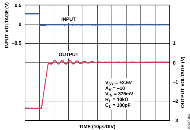
Figure 47. Negative Overload Recovery
