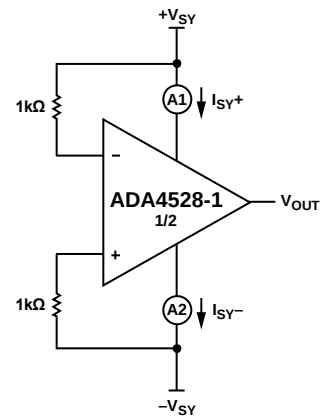
Figure 67. Comparator A
