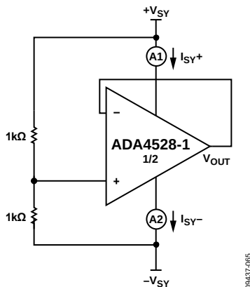
Figure 65. Voltage Follower
