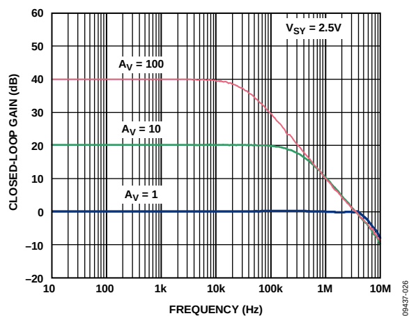
Figure 27. Closed-Loop Gain vs. Frequency
