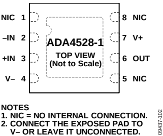
Figure 5. ADA4528-1 Pin Configuration, 8-Lead LFCSP
