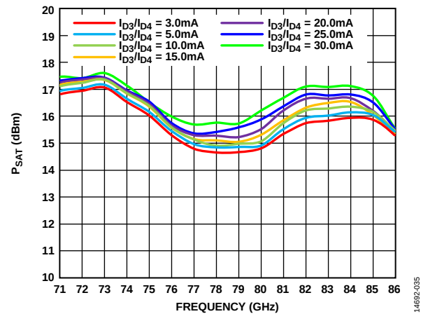
Figure 35. Saturated Output Power ( P_{SAT} ) vs. Frequency over Drain Current, V_{Dx} = 4\text{ V} , V_{G1} and V_{G2} Fixed at 20 mA, V_{G3} and V_{G4} Swept
