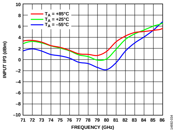
Figure 34. Input Third-Order Intercept (IP3) vs. Frequency over Temperature, V_{Dx} = 4\text{ V} , I_{Dx} = 50\text{ mA}
