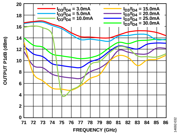
Figure 32. Output P1dB vs. Frequency over Drain Current, V_{Dx} = 4\text{ V} , V_{G1} and V_{G2} Fixed at 20 mA, V_{G3} and V_{G4} Swept
