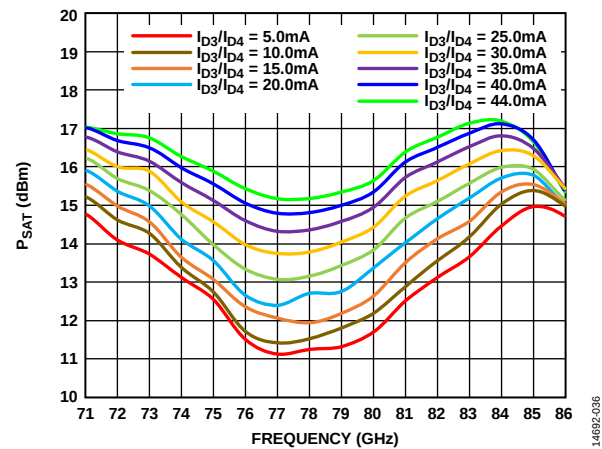
Figure 36. Saturated Output Power ( P_{SAT} ) vs. Frequency over Drain Current, V_{D1} and V_{D2} = 2\text{ V} , V_{D3} and V_{D4} = 4\text{ V}
