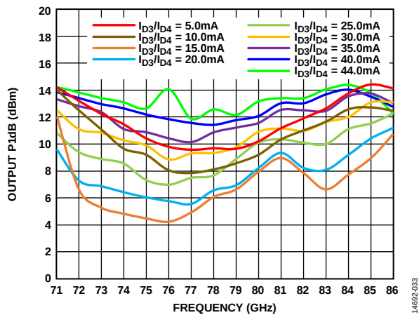
Figure 33. Output P1dB vs. Frequency over Drain Current, V_{D1} and V_{D2} = 2\text{ V} , V_{D3} and V_{D4} = 4\text{ V}
