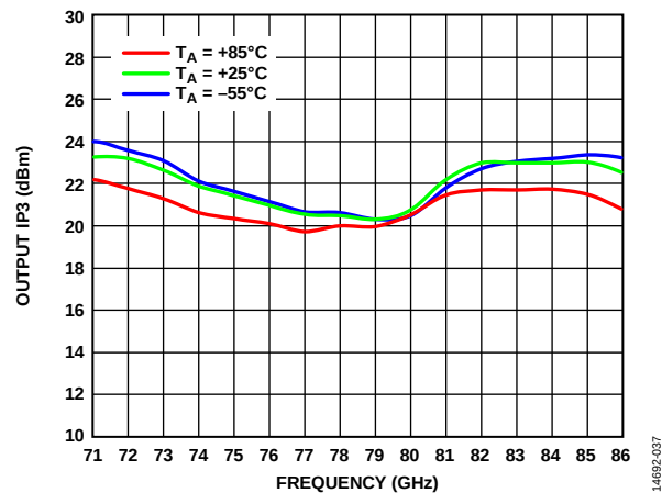
Figure 37. Output Third-Order Intercept (IP3) vs. Frequency over Temperature, V_{Dx} = 4\text{ V} , I_{Dx} = 50\text{ mA}
