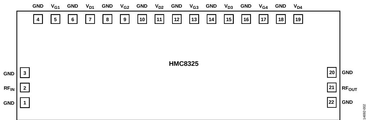
Figure 2. Pin Configuration
