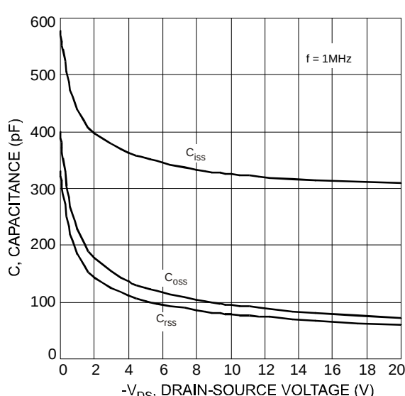
Fig. 6 Typical Capacitance
