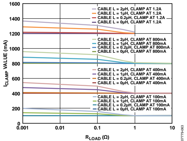
Figure 53. I_{CLAMP} Value vs. R_{LOAD} - Cal at 10Ohm
