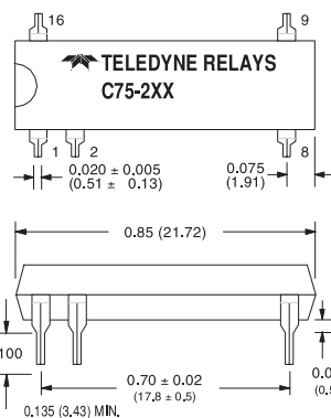
DIMENSIONS ARE IN INCHES (MILLIMETERS) Tolerances ± 0.015 (0.38) unless specified.
