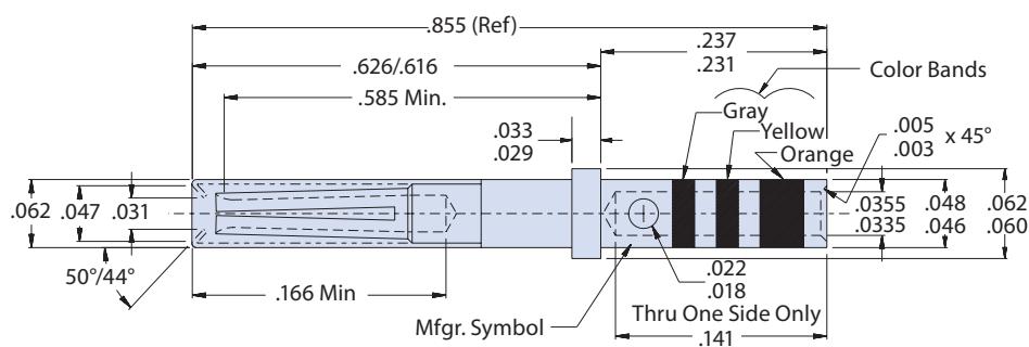
Socket Contact
