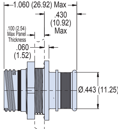
801-084-07 Jam Nut Mount Receptacle with Shield Termination Porch
