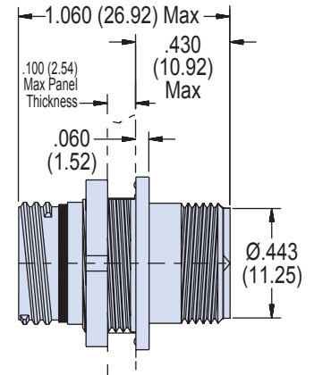
801-085-07 Jam Nut Mount Receptacle with Accessory Threads
