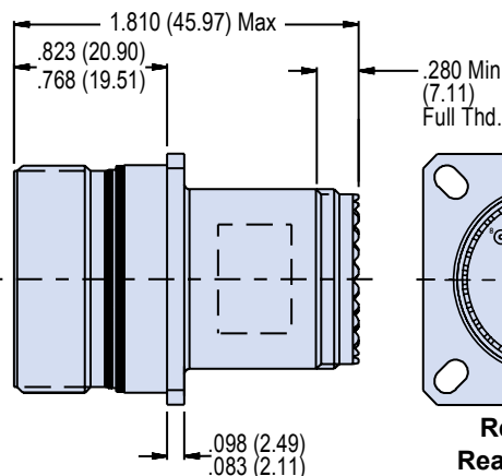
Square Flange Mount Receptacle
