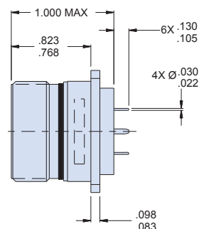
Square Flange Receptacle
